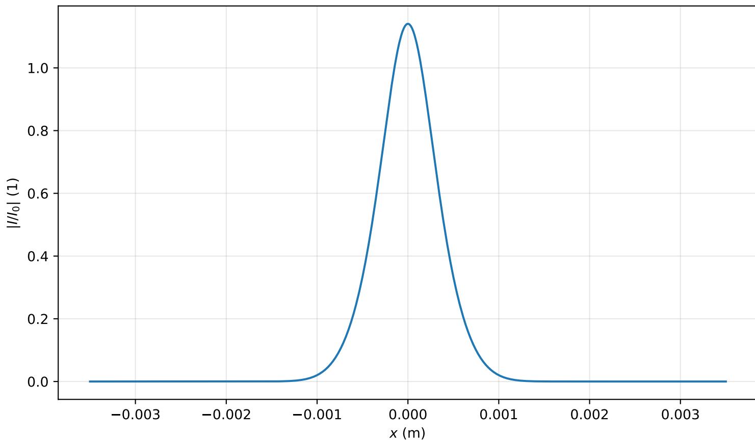
Intensity profile I(x, y = 0, z = 0.557m)/I_0 , P_{in}=0.8P_{cr} , artificial time
